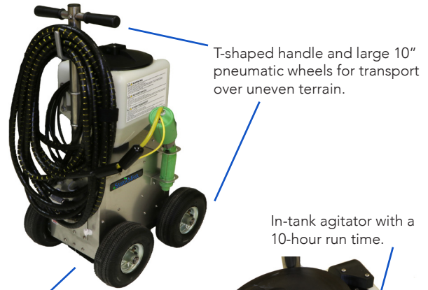
A grounding plate helps ensure effective transfer into uniform droplets.
