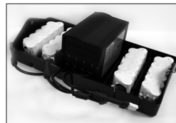
The charger sequentially recharges two sets of batteries. It restores 60% capacity in 60 minutes, 90% in 90 minutes, and fully recharges a set in two hours. The tray simplifies staging in large facilities.
